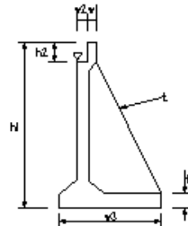
躯体工(2)
