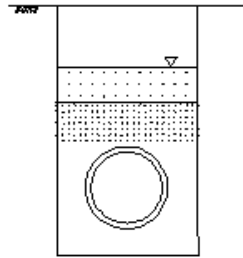
管路埋戻
