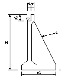
躯体工(2)
