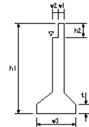
躯体工(3)
