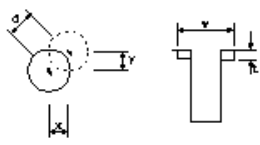
集水井工 d = \sqrt{R^2 + Y^2}
