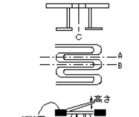
expansion device (steel finger joint)
