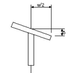
precast girder work (flange perpendicularity)
