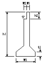
躯体工(3)
