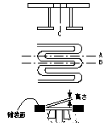
expansion device (steel finger joint)
