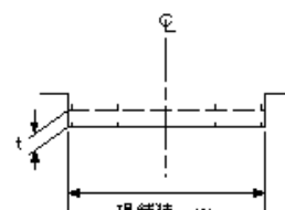
road cutting
