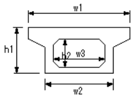
PC push-out box girder construction
