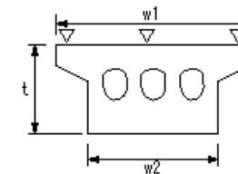
PC hollow slab construction
