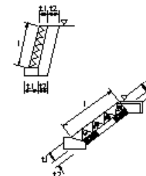
concrete block construction (concrete block stacking) (concrete block stacking)
