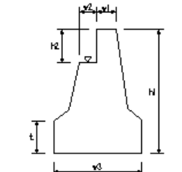
躯体工(1)
