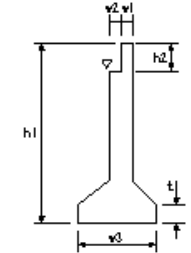
躯体工(3)
