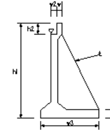
躯体工(2)
