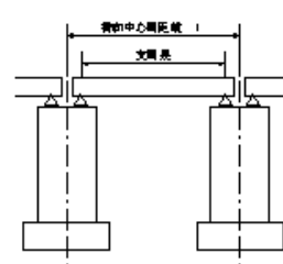
RC躯体工
