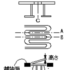
expansion device (steel finger joint)
