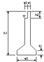
躯体工(3)
